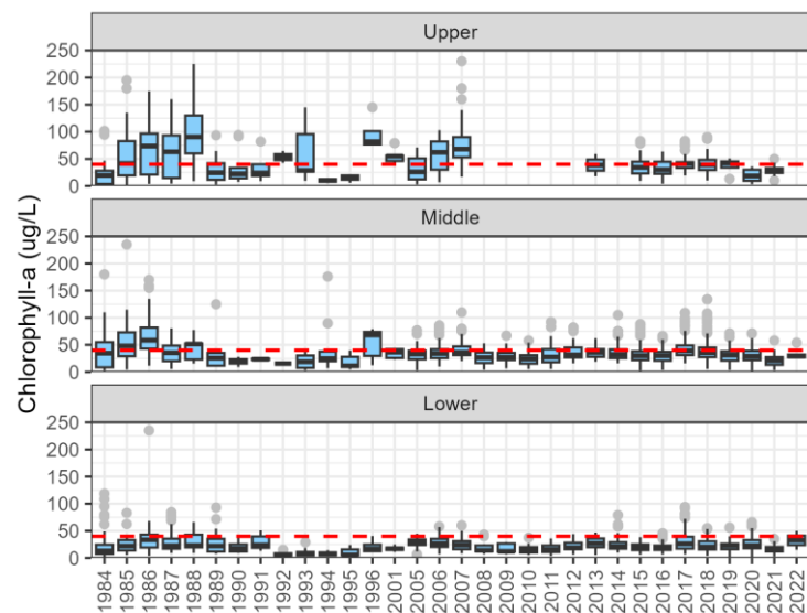
Figure 5. Distribution of Chlorophyll-a Measurements in Upper Falls Lake (upstream of Interstate 85), Middle Falls Lake (between Interstate 85 and Highway 50) and Lower Falls Lake (downstream of Highway 50 to the Dam)
